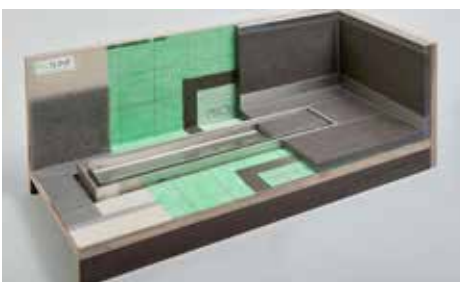
PROCHANNEL s -line with tile recess Item No.: M31468 (Size: 508 x 210 x 198 mm)
