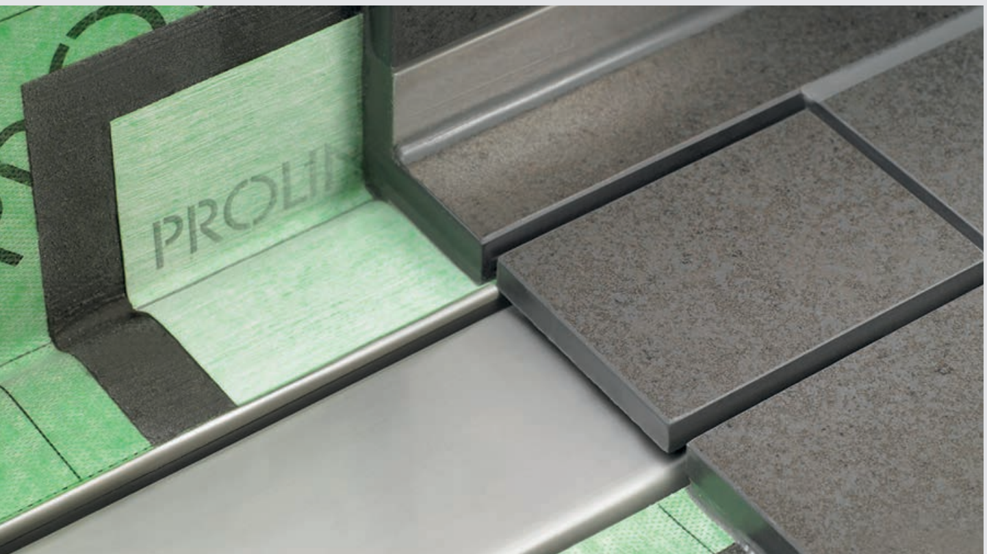
PROCHANNELs-line carrier element with glued tile to create a shadow gap.
