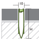
Design close to surface | Surface peu excavé
