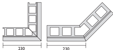
External corner 90° | Angle sortant 90° External corner 135° | Angle sortant 135°
