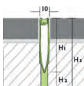
Design close to surface | Surface peu excavé
