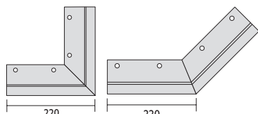
External corner 90° | External corner 135° Angle sortant 90° | Angle sortant 135°
