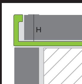
PROFLOOR
