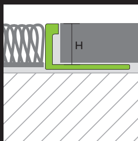
PROCURVE
