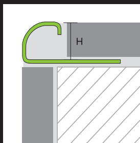
PROROUND Edelstahl
