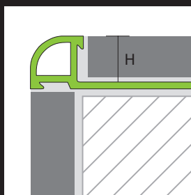
PROROUND Aluminium/PVC
